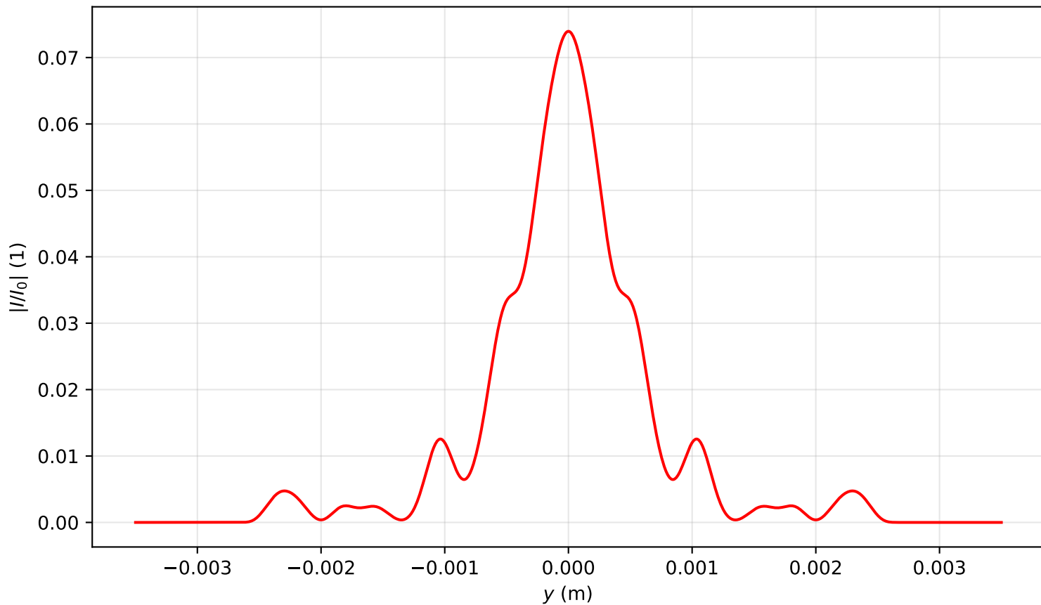
Intensity profile I(x=0, y, z=3.662)/I_0 , P_{in}=8.0P_{cr} , artificial time
